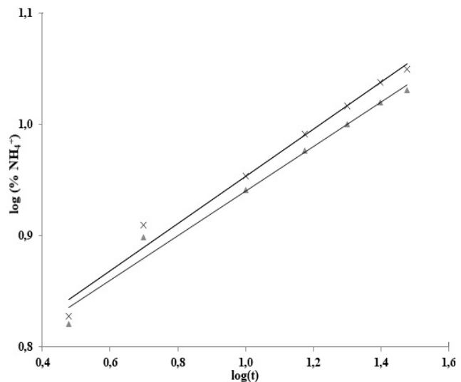
Figure 3 Adjustment to the Korsmeyer-Peppas model for the release of NH 4 + in water: Δ hydrogel in soil, ×hydrogel in sand.
