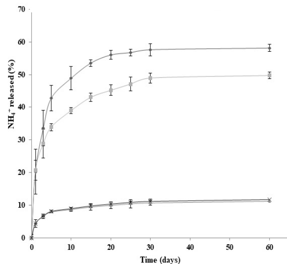
Figure 2 Release of NH4+ in water: ◆ diammonium phosphate in soil, ■ diammonium phosphate in sand; ▲ hydrogel in soil, × hydrogel in sand. Source: The authors
